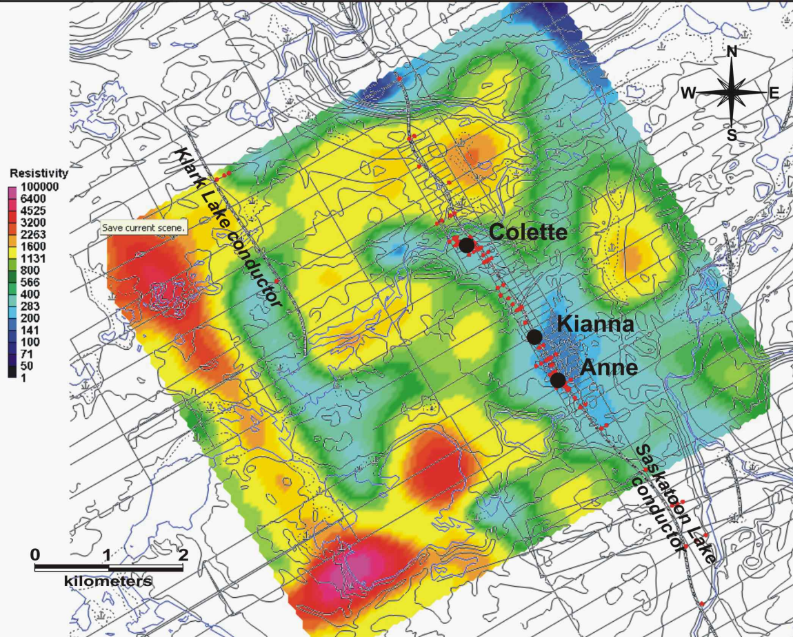
Contoured DC-resistivity inverted horizontal depth slice at -350 m below sea level for the northern Shea Creek and southernmost Douglas River properties.
