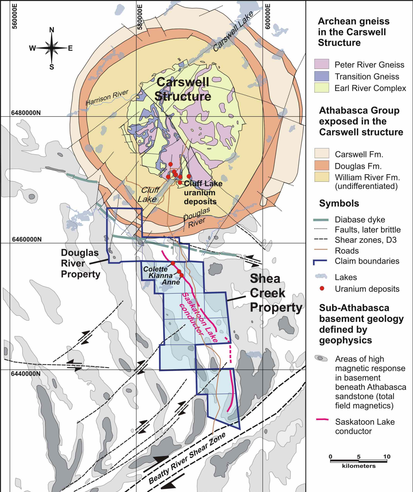
Geological setting of the Shea Creek property
