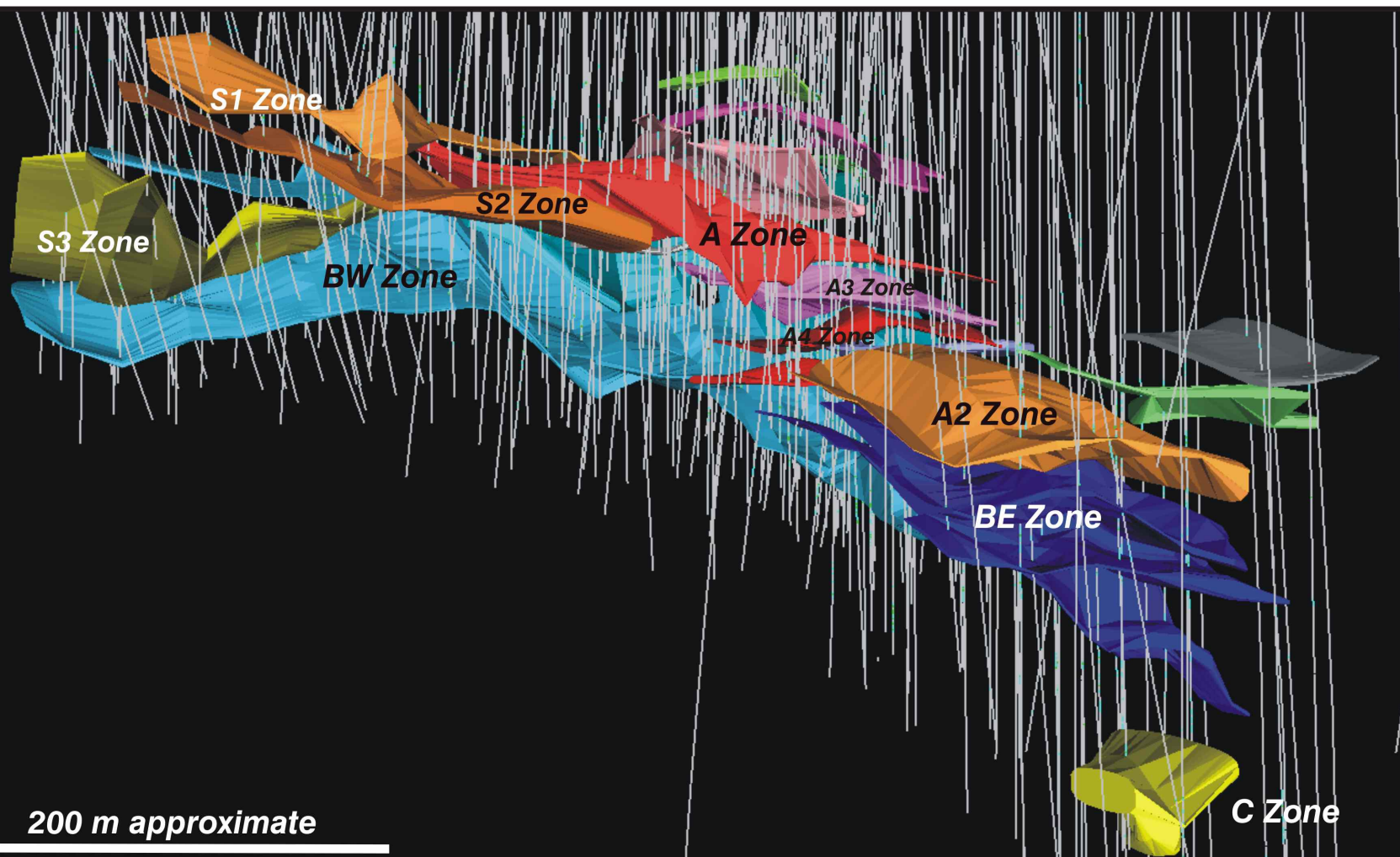
Horseshoe Deposit, 3-D wireframe model viewed from the southwest, looking northwest
