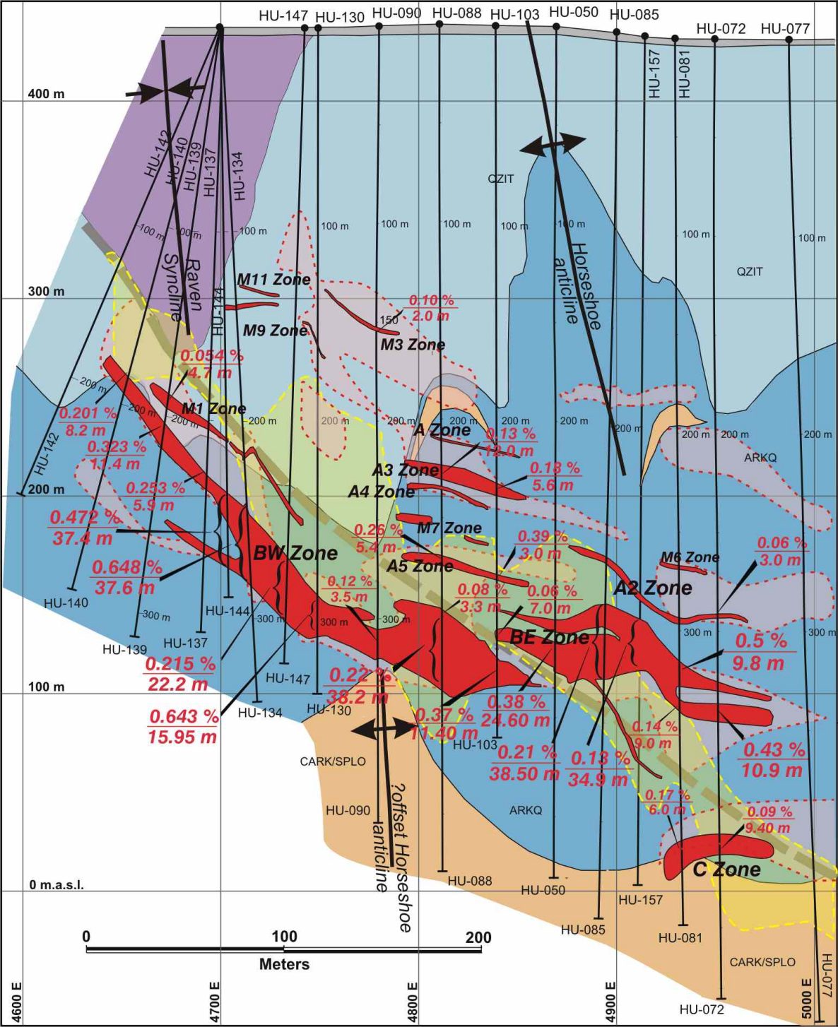
Horseshoe Deposit Section 4724N Looking northeast
