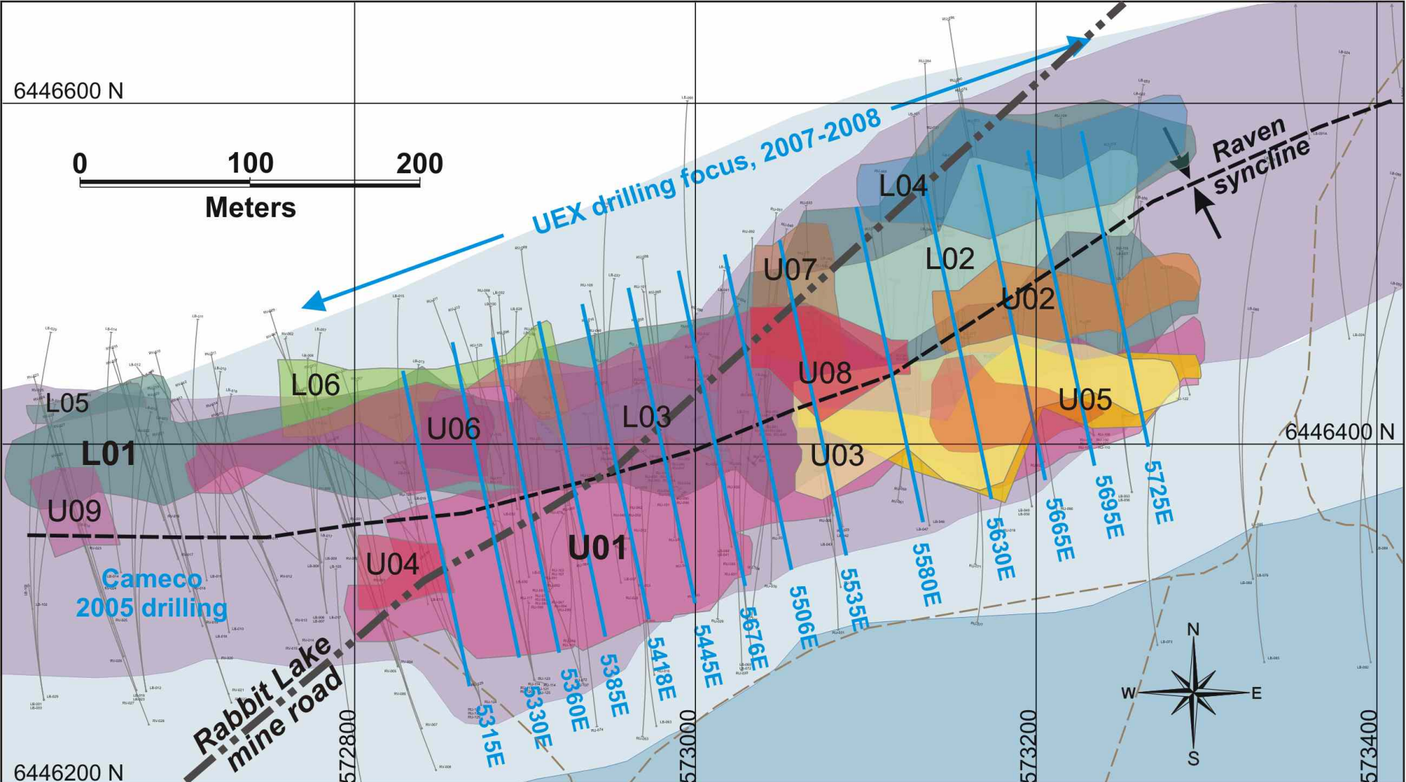
Raven Deposit geology map, showing plan view projected outlines of mineralized zones modeled using Datamine software. U-series sub-zones refer to the Upper Zone, while L-series sub-zones refer to the Lower Zone
