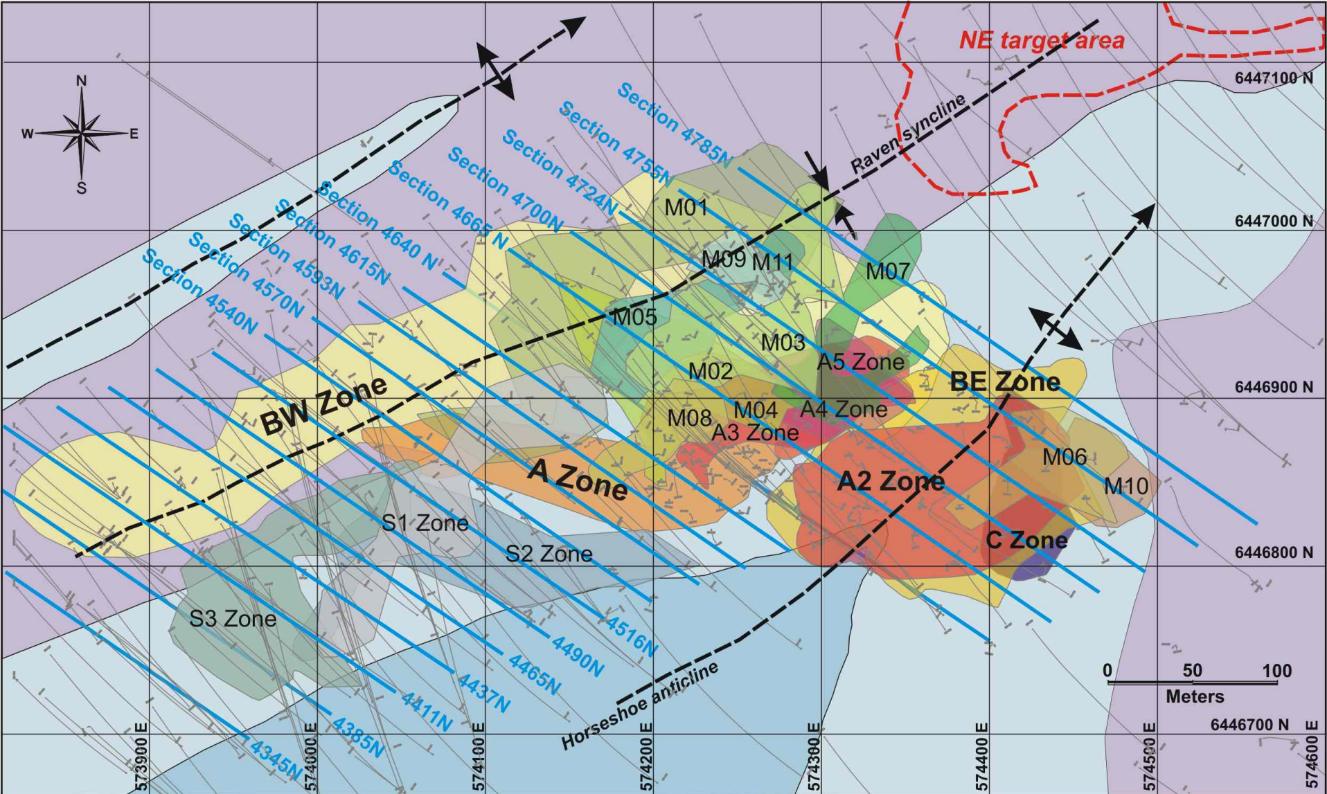
Geological plan map of the Horseshoe deposit, showing surface projection of mineralized zones and surface geology, based on drilling data.
