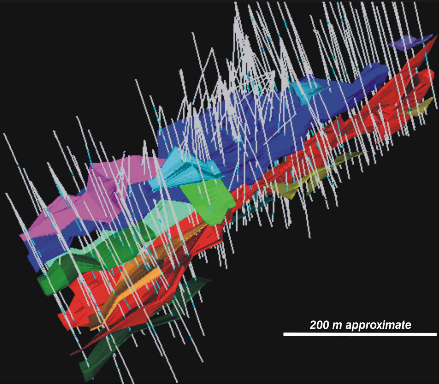
Raven Deposit, 3-D wireframe model viewed from the northeast, looking southwest
